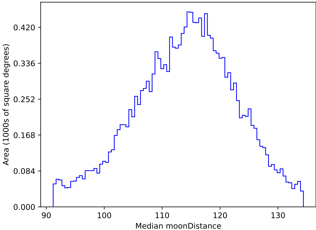
mw_roll_bulge_v3.3_10yrs WFD g band: Median moonDistance
