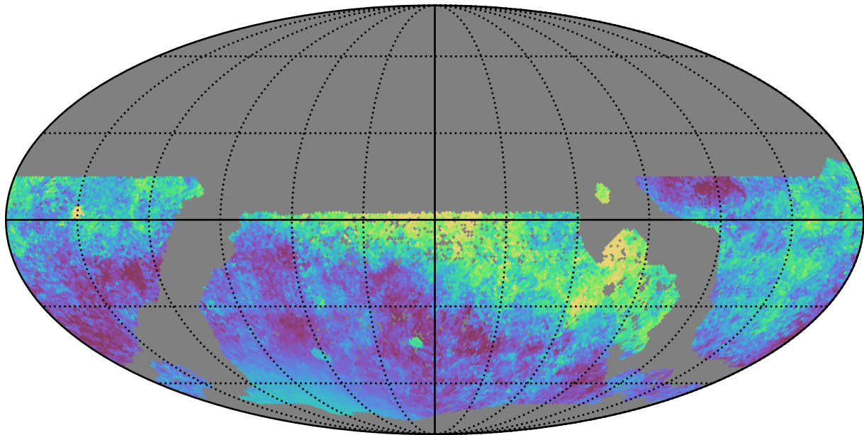
mw_roll_bulge_v3.3_10yrs WFD all bands: Median moonDistance
