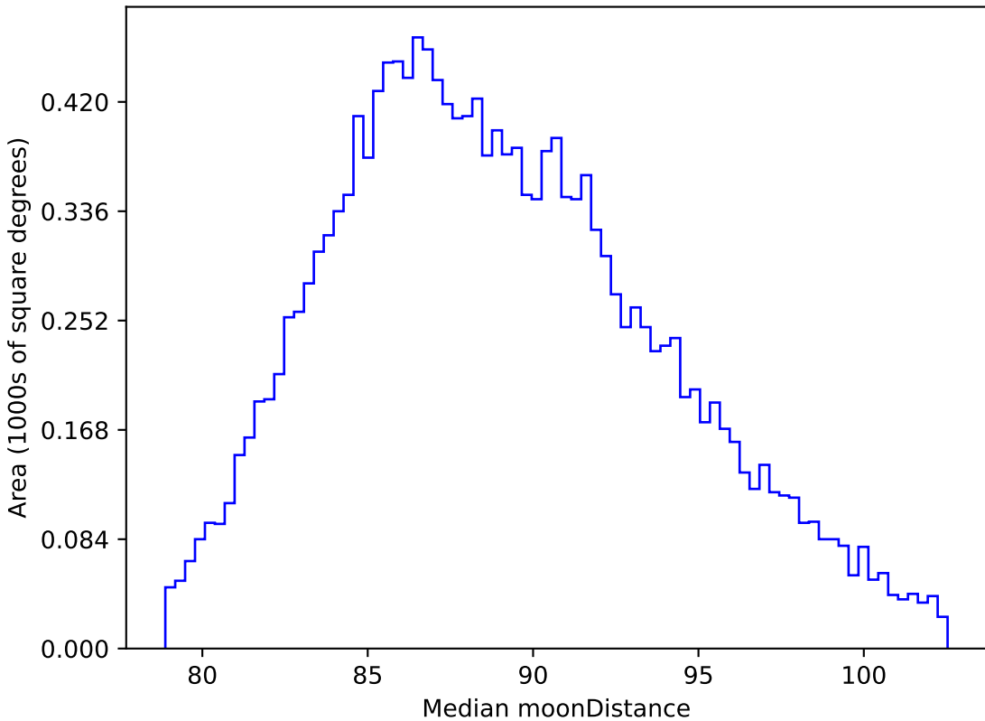
mw_roll_bulge_v3.3_10yrs WFD all bands: Median moonDistance
