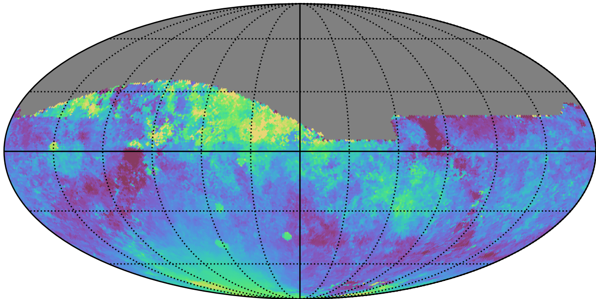
mw_roll_bulge_v3.3_10yrs All sky z band: Median moonDistance
