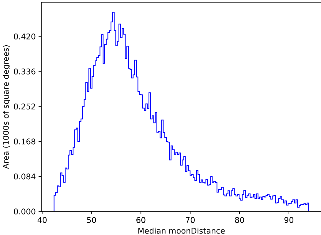
mw_roll_bulge_v3.3_10yrs All sky y band: Median moonDistance
