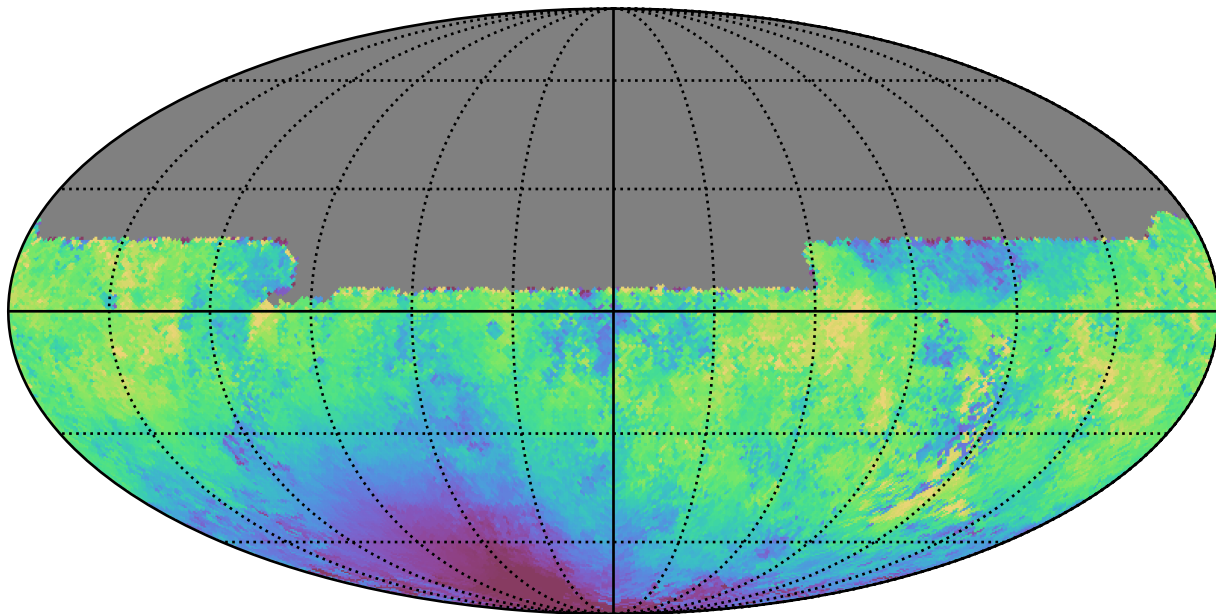
mw_roll_bulge_v3.3_10yrs All sky u band: Median moonDistance
