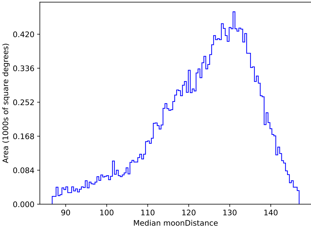
mw_roll_bulge_v3.3_10yrs All sky u band: Median moonDistance
