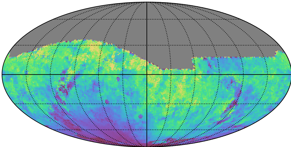
mw_roll_bulge_v3.3_10yrs All sky r band: Median moonDistance
