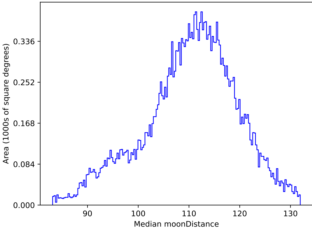
mw_roll_bulge_v3.3_10yrs All sky r band: Median moonDistance
