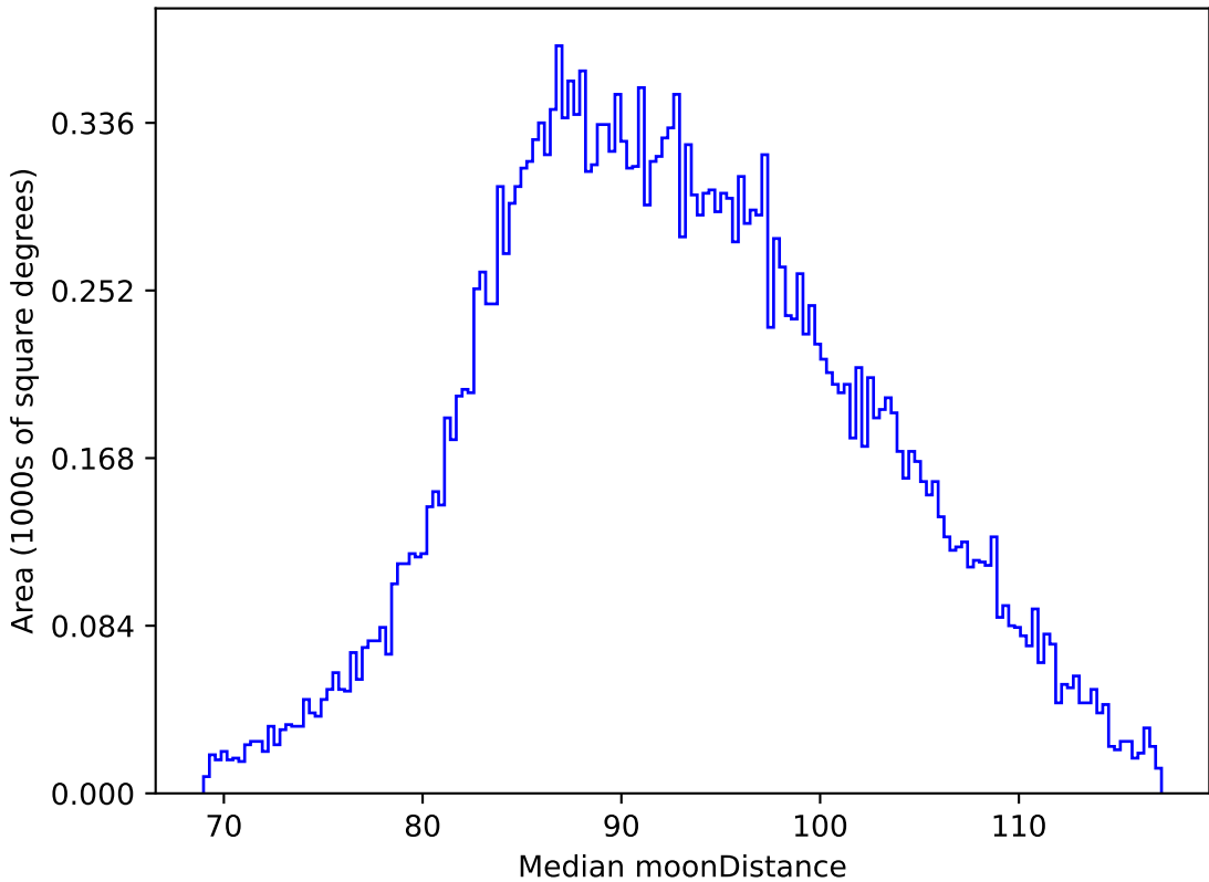
mw_roll_bulge_v3.3_10yrs All sky i band: Median moonDistance
