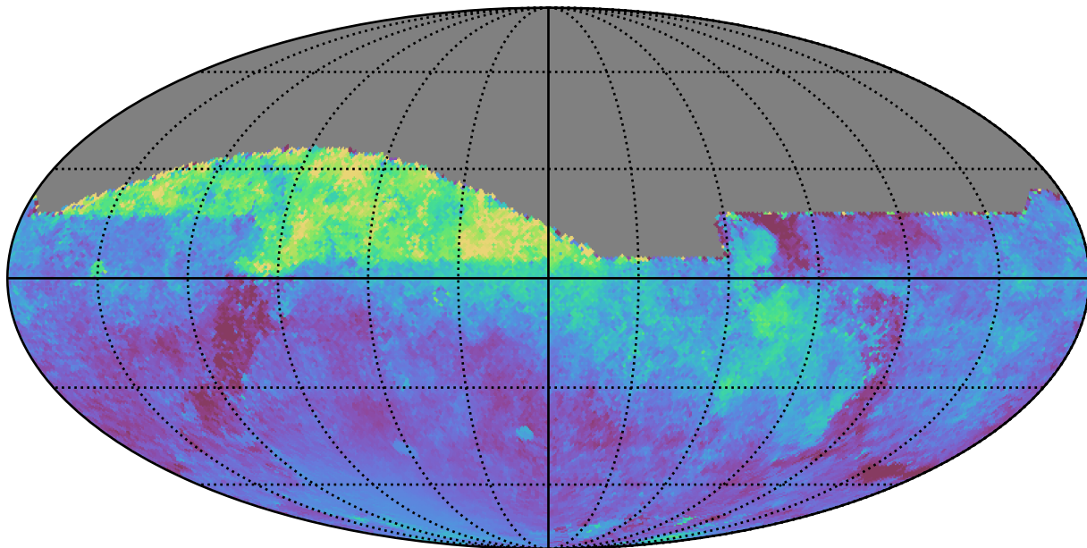
mw_roll_bulge_v3.3_10yrs All sky all bands: Median moonDistance
