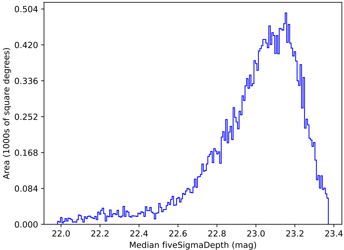
mw_roll_bulge_v3.3_10yrs Yr 1 z band: Median fiveSigmaDepth
