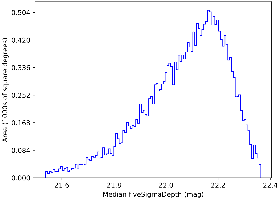
mw_roll_bulge_v3.3_10yrs Yr 1 y band: Median fiveSigmaDepth
