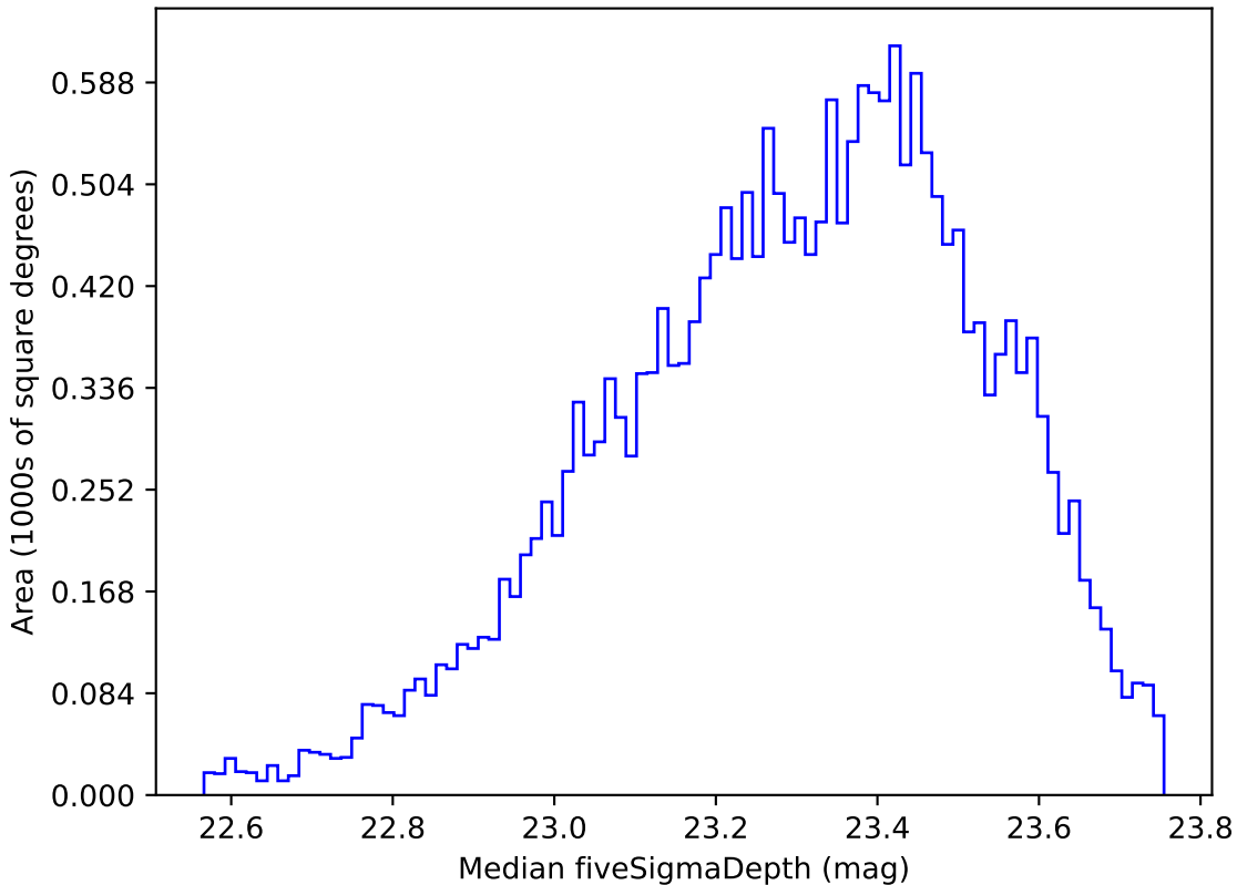
mw_roll_bulge_v3.3_10yrs Yr 1 u band: Median fiveSigmaDepth
