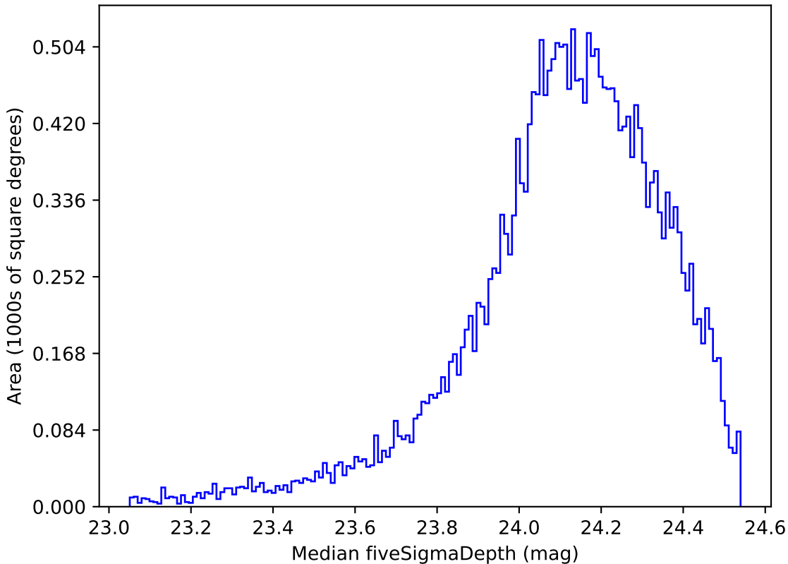
mw_roll_bulge_v3.3_10yrs Yr 1 r band: Median fiveSigmaDepth
