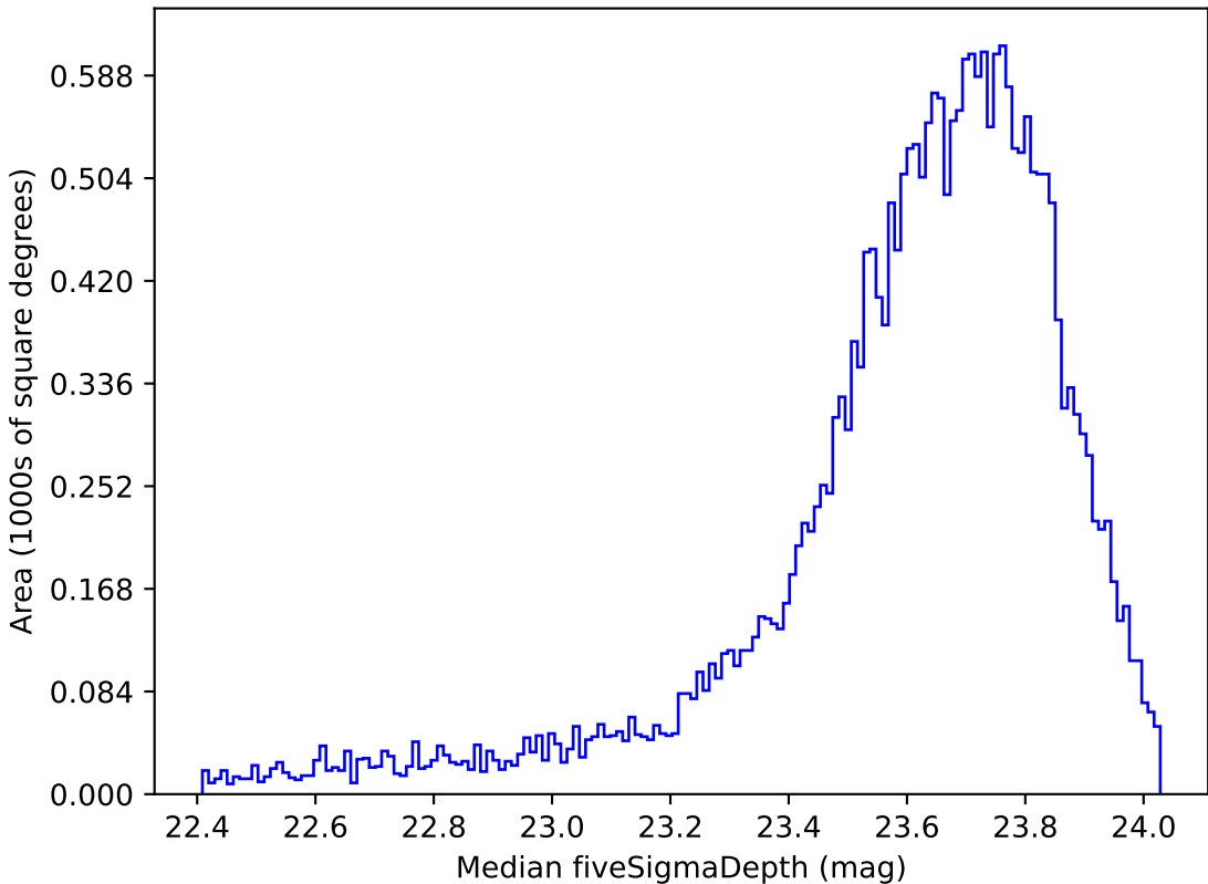
mw_roll_bulge_v3.3_10yrs Yr 1 i band: Median fiveSigmaDepth
