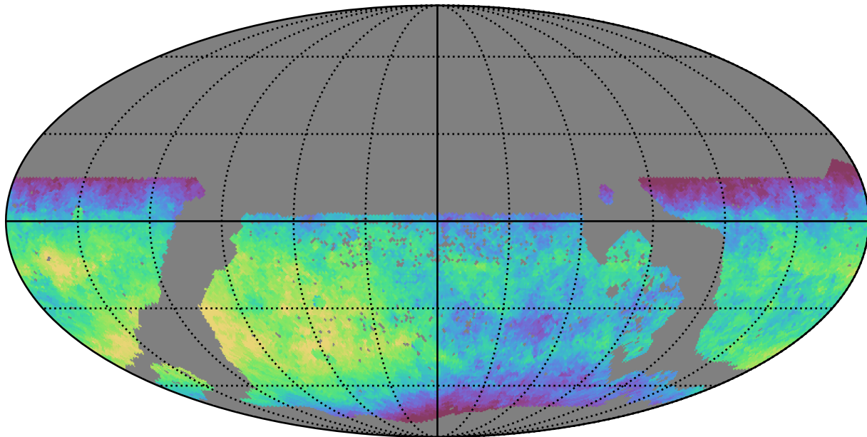
mw_roll_bulge_v3.3_10yrs WFD z band: Median fiveSigmaDepth
