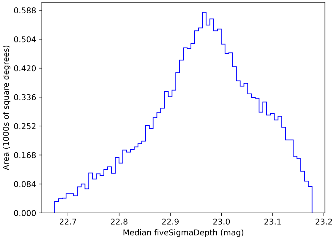
mw_roll_bulge_v3.3_10yrs WFD z band: Median fiveSigmaDepth
