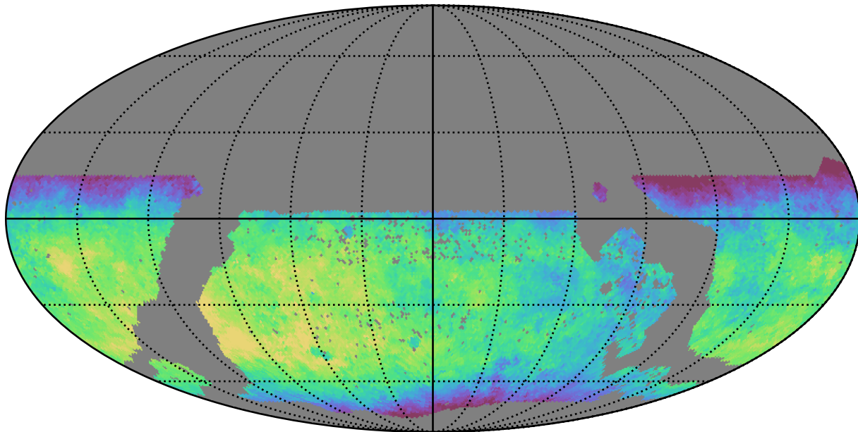
mw_roll_bulge_v3.3_10yrs WFD y band: Median fiveSigmaDepth
