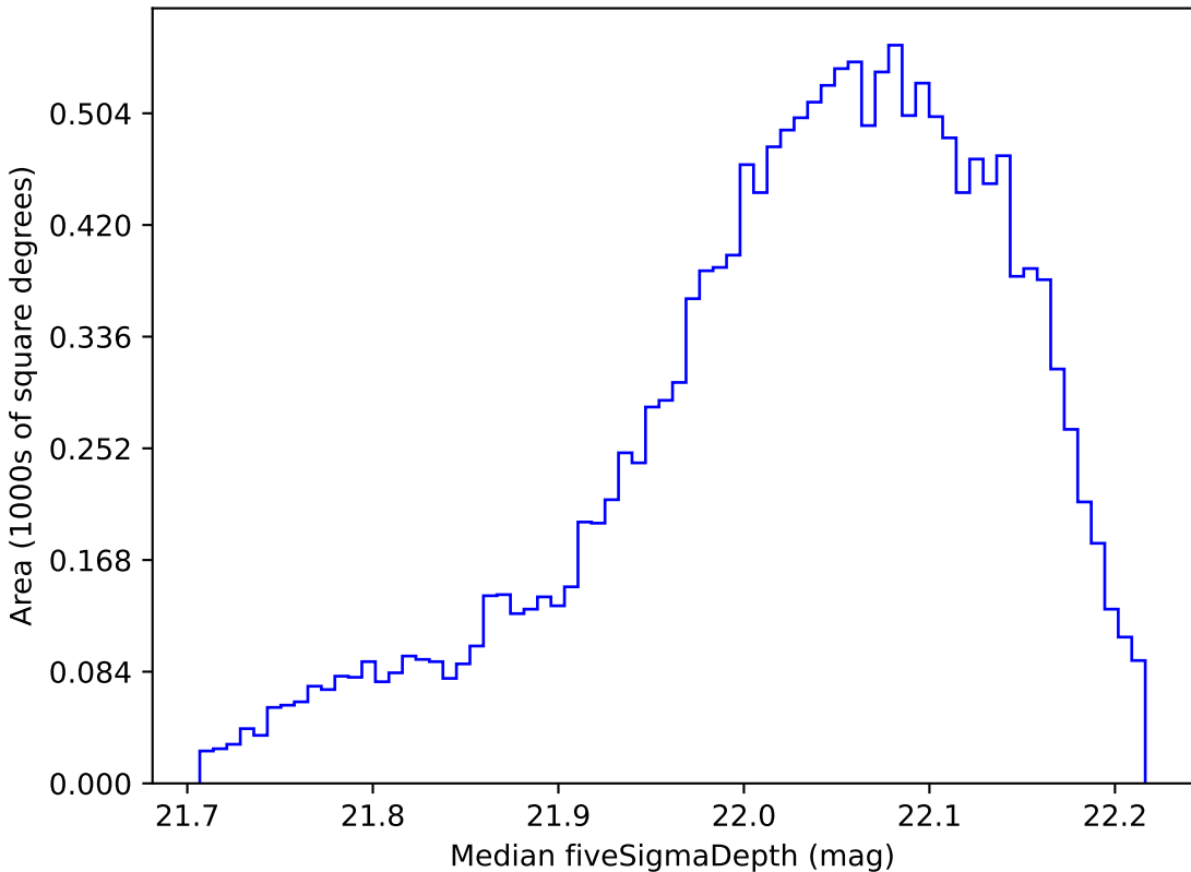
mw_roll_bulge_v3.3_10yrs WFD y band: Median fiveSigmaDepth
