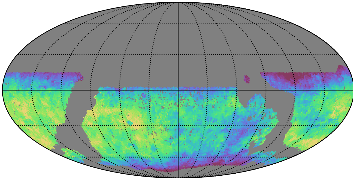
mw_roll_bulge_v3.3_10yrs WFD u band: Median fiveSigmaDepth
