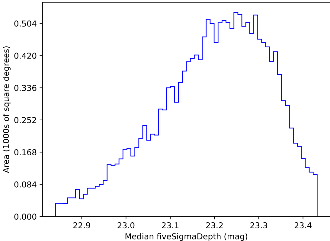
mw_roll_bulge_v3.3_10yrs WFD u band: Median fiveSigmaDepth
