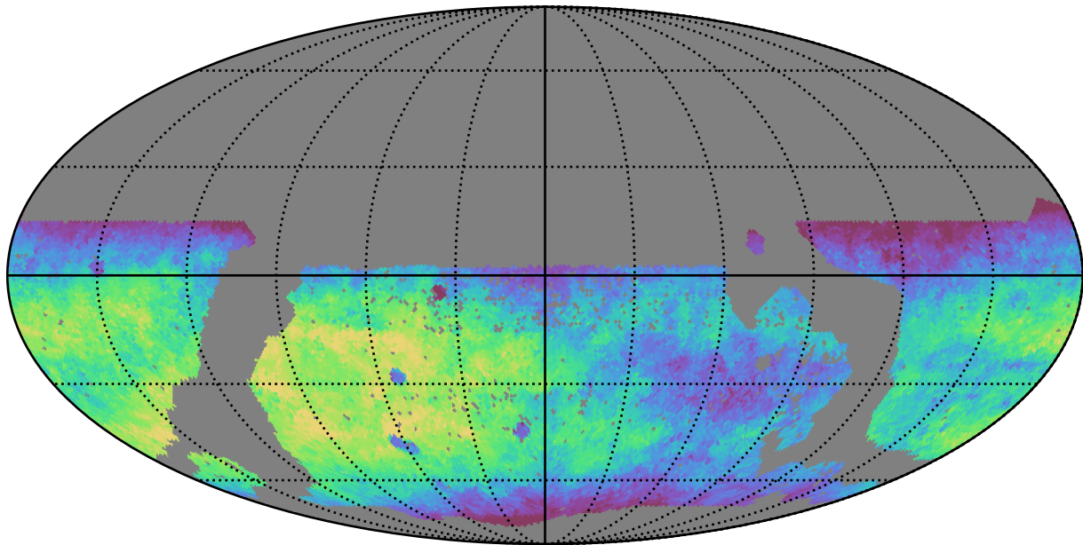
mw_roll_bulge_v3.3_10yrs WFD r band: Median fiveSigmaDepth
