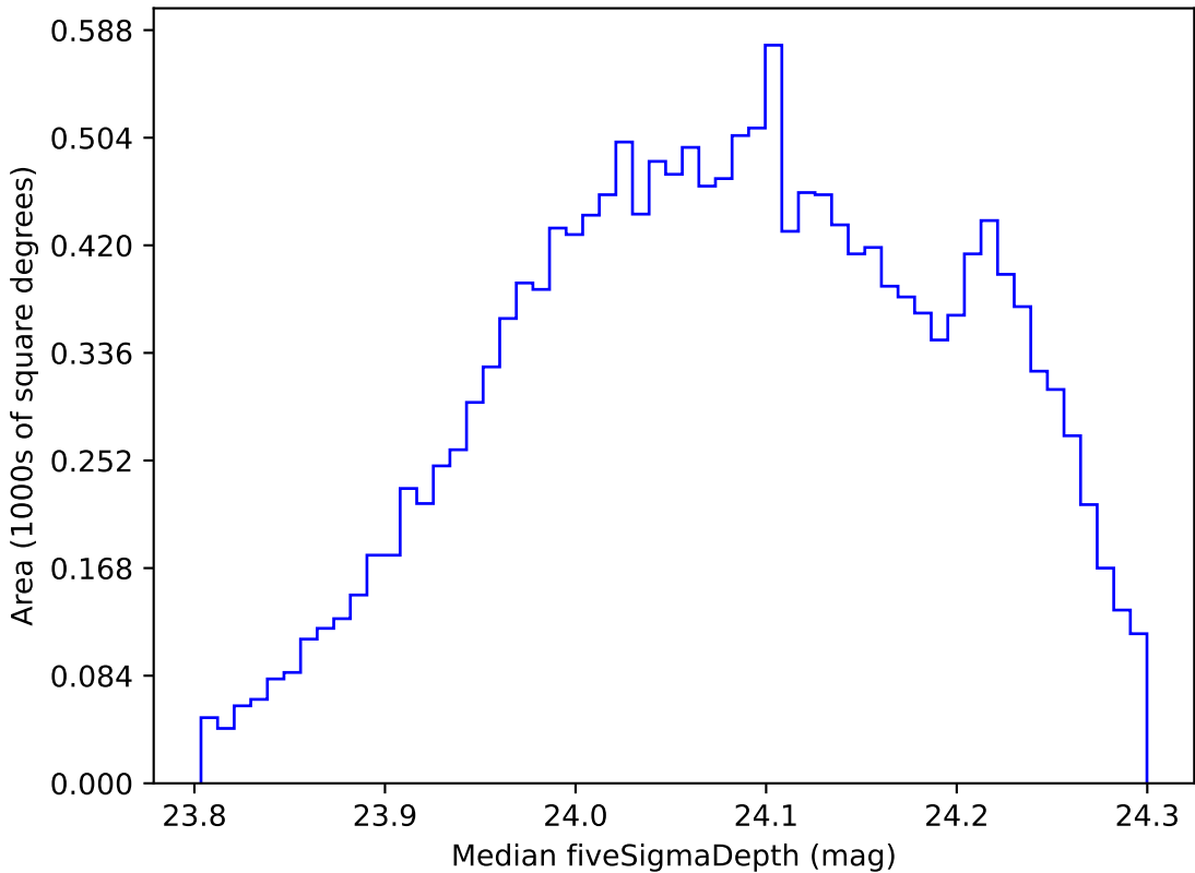
mw_roll_bulge_v3.3_10yrs WFD r band: Median fiveSigmaDepth
