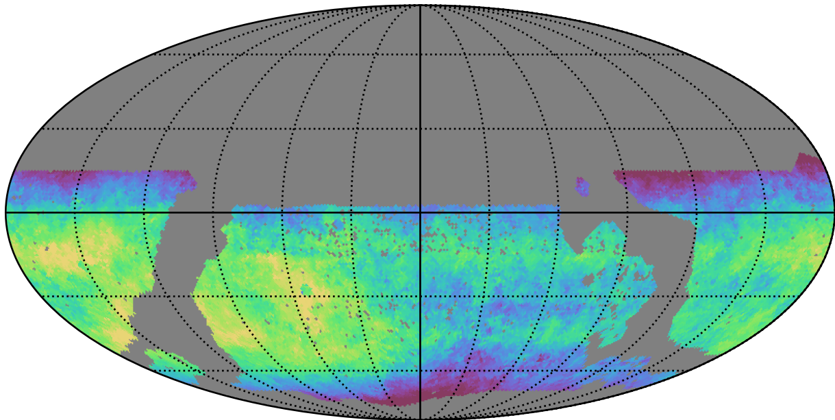
mw_roll_bulge_v3.3_10yrs WFD i band: Median fiveSigmaDepth
