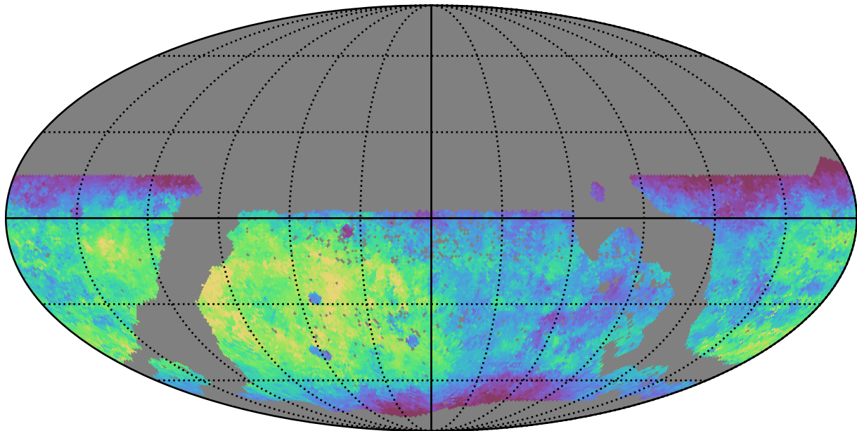
mw_roll_bulge_v3.3_10yrs WFD g band: Median fiveSigmaDepth
