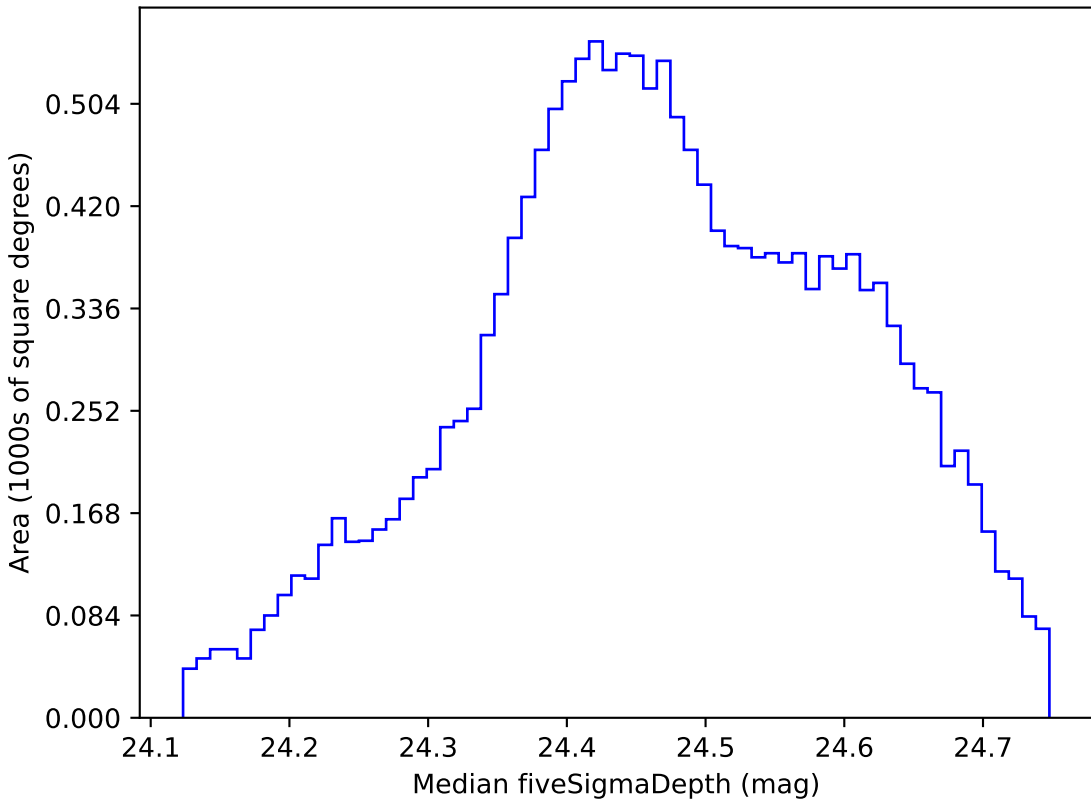
mw_roll_bulge_v3.3_10yrs WFD g band: Median fiveSigmaDepth
