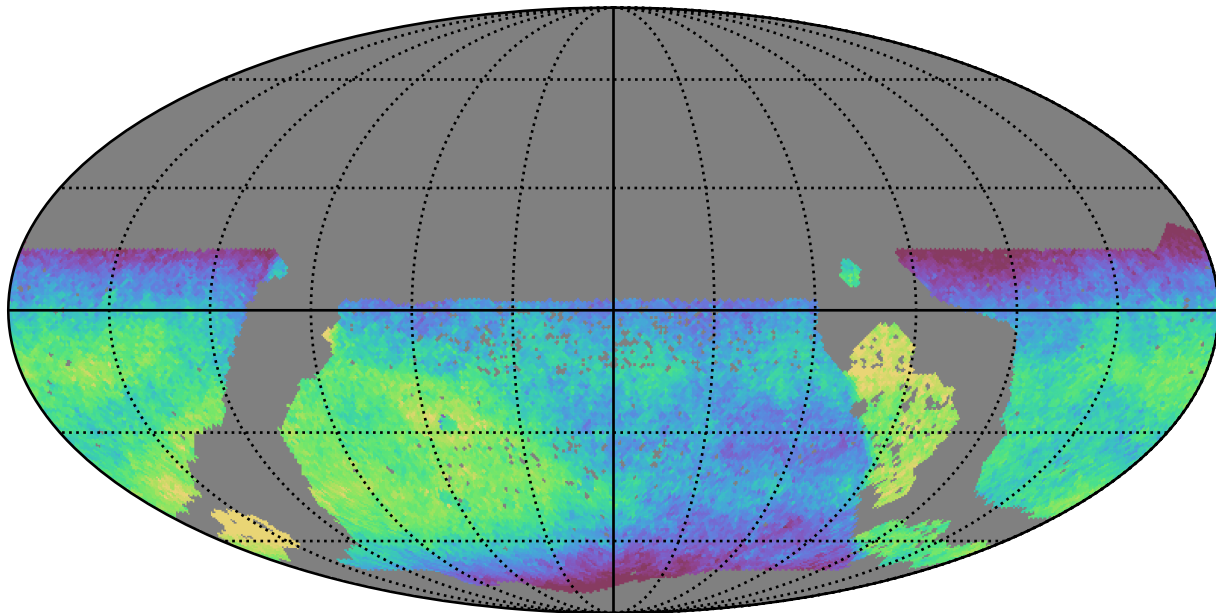
mw_roll_bulge_v3.3_10yrs WFD all bands: Median fiveSigmaDepth
