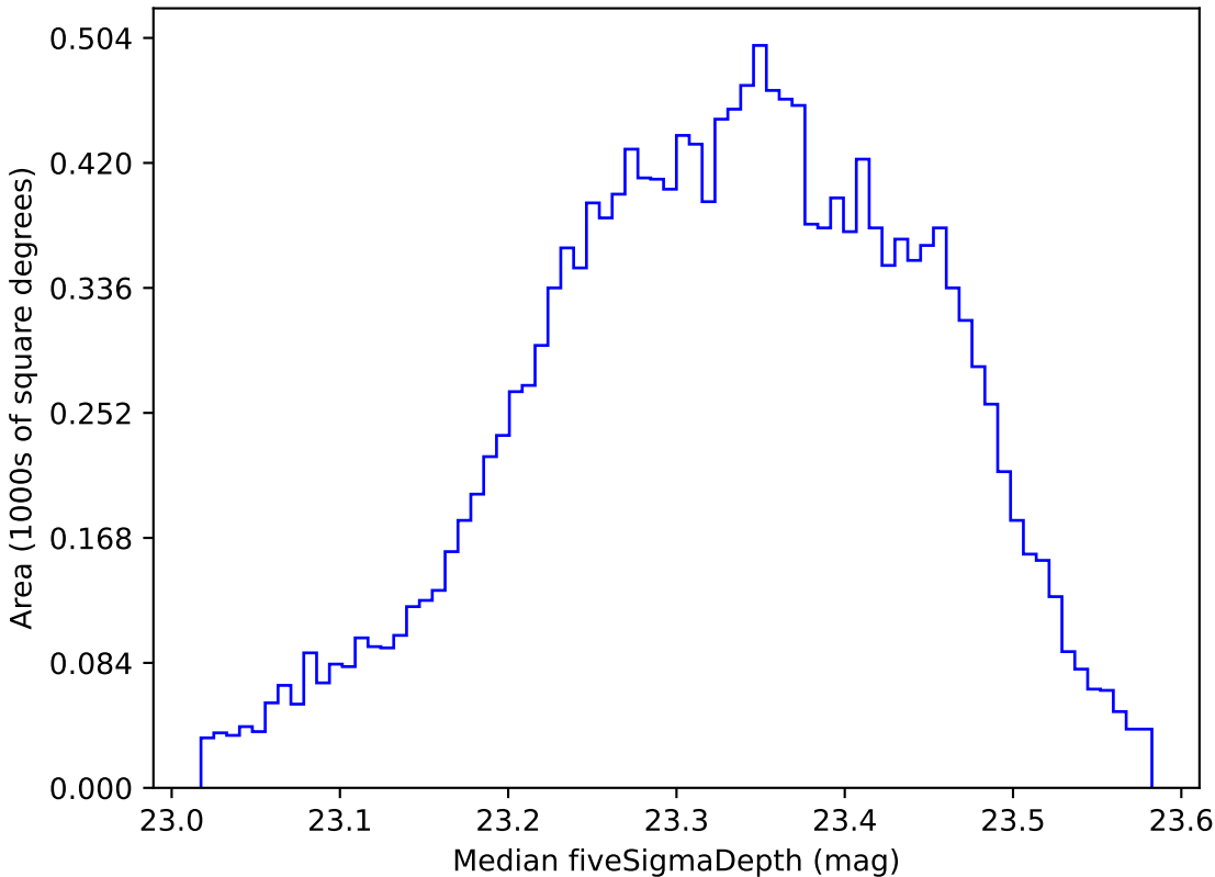
mw_roll_bulge_v3.3_10yrs WFD all bands: Median fiveSigmaDepth
