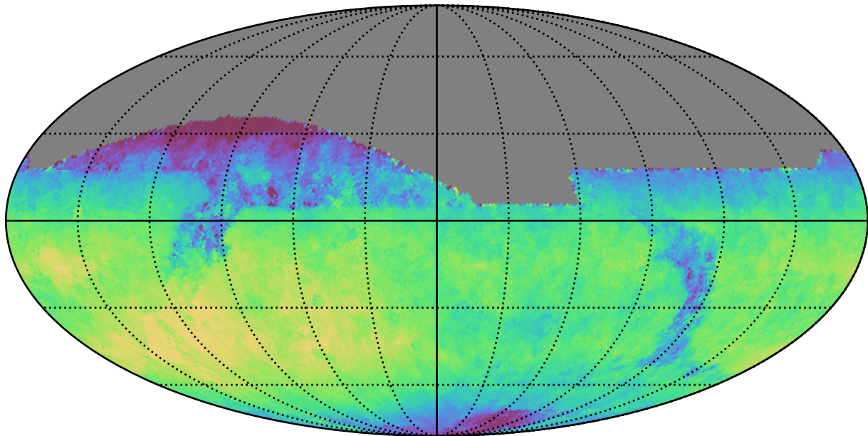
mw_roll_bulge_v3.3_10yrs All sky z band: Median fiveSigmaDepth
