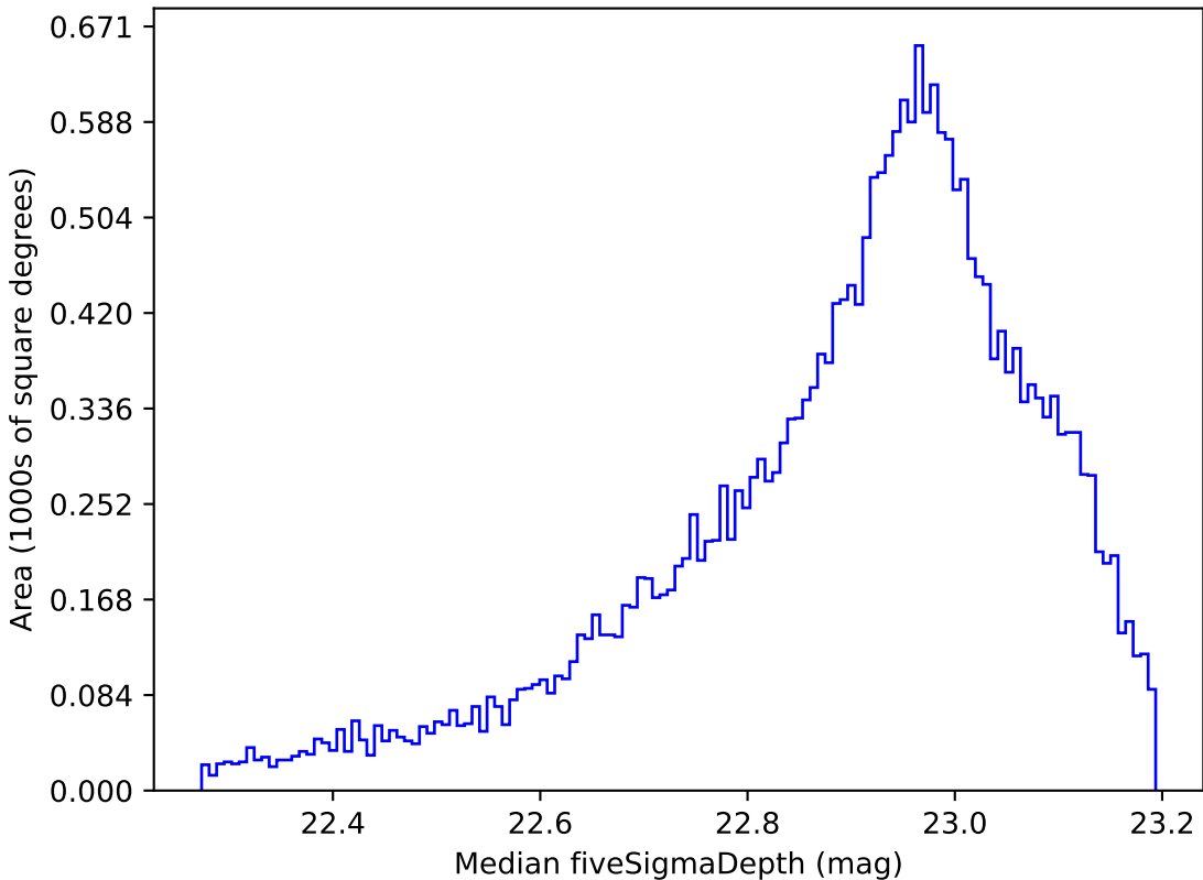
mw_roll_bulge_v3.3_10yrs All sky z band: Median fiveSigmaDepth
