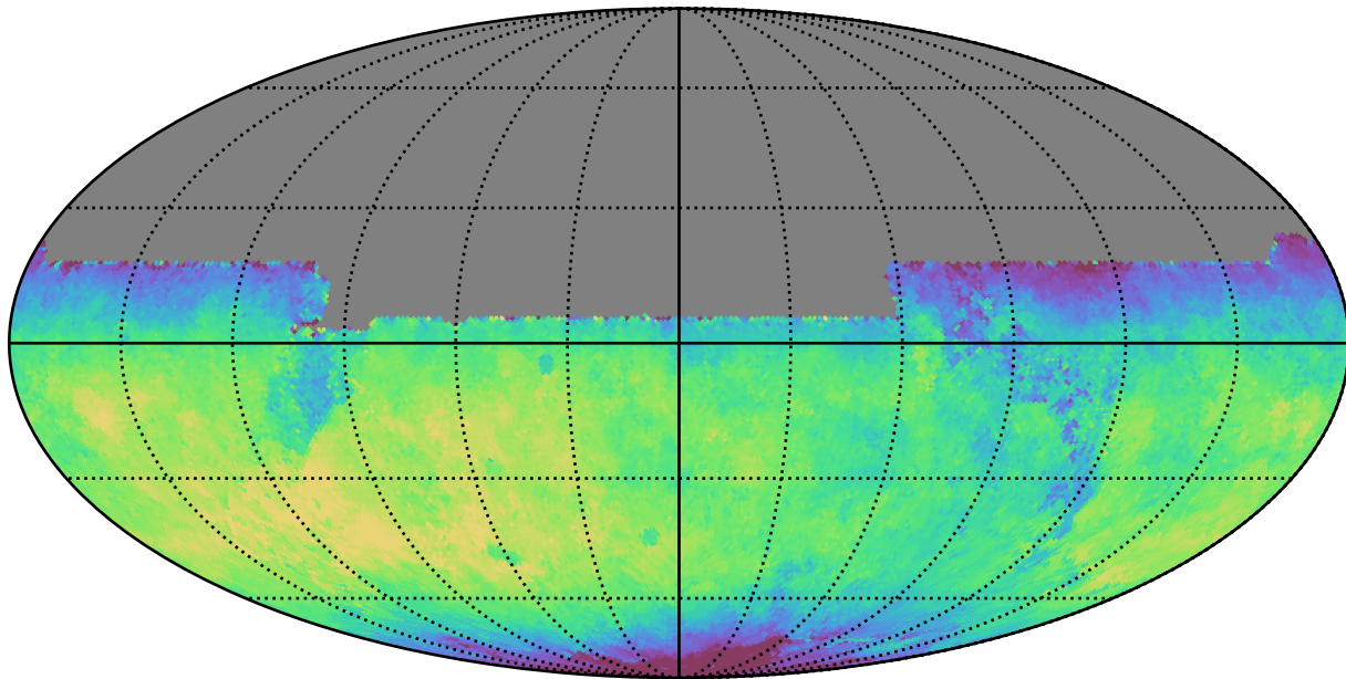
mw_roll_bulge_v3.3_10yrs All sky y band: Median fiveSigmaDepth
