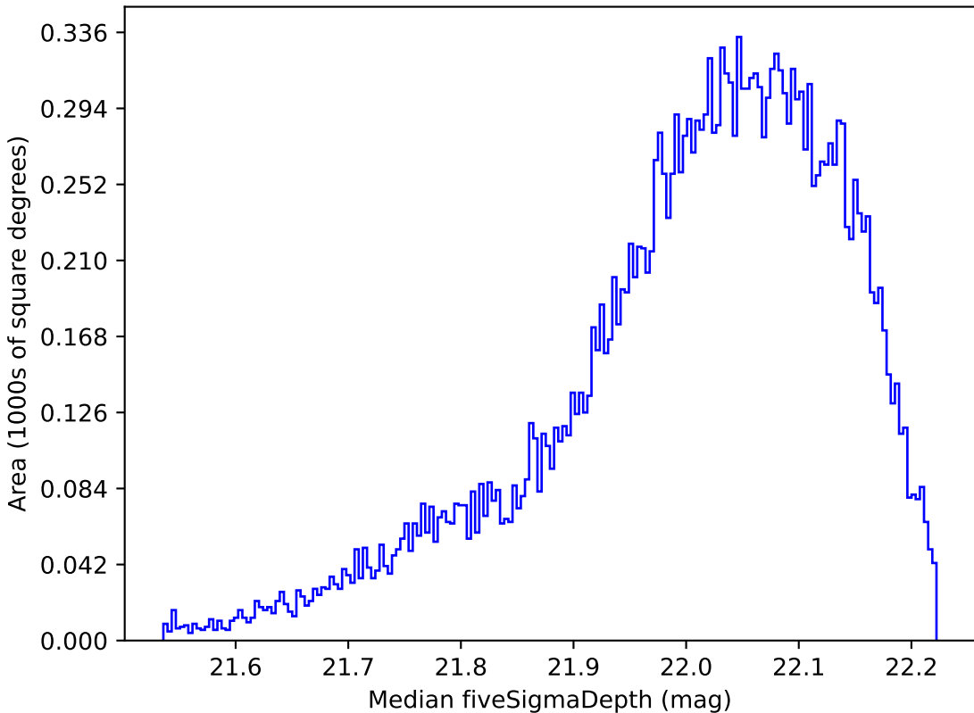
mw_roll_bulge_v3.3_10yrs All sky y band: Median fiveSigmaDepth
