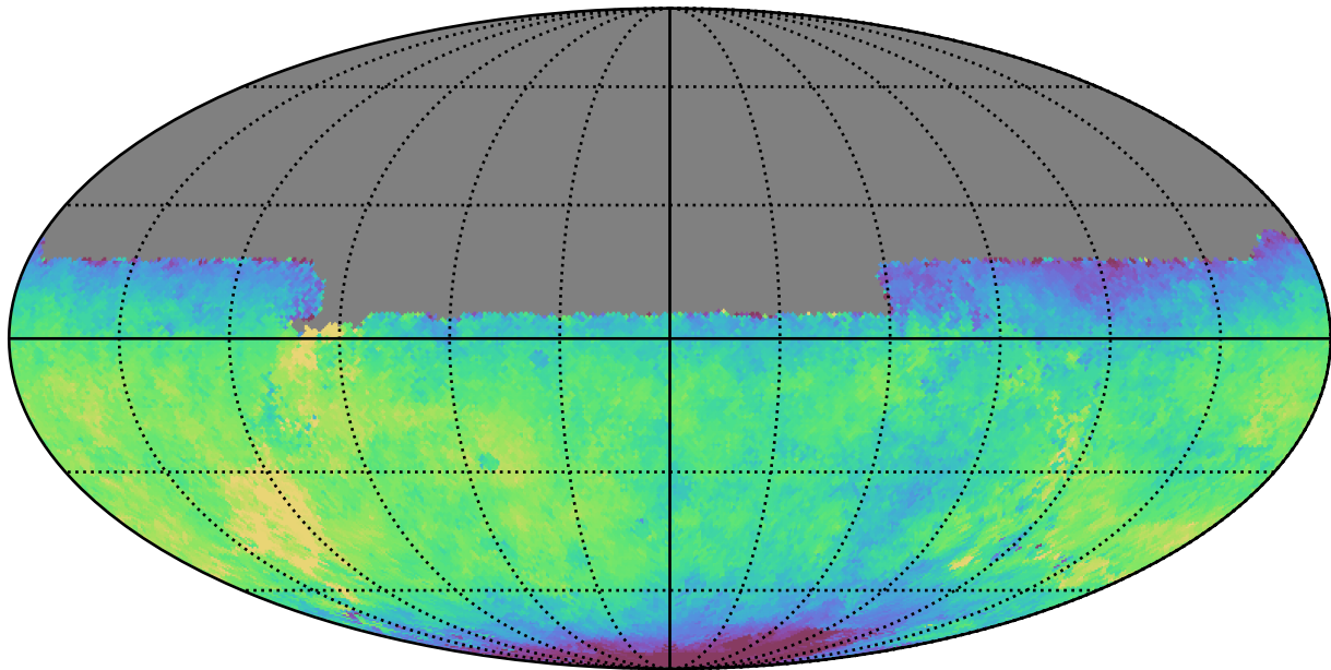
mw_roll_bulge_v3.3_10yrs All sky u band: Median fiveSigmaDepth
