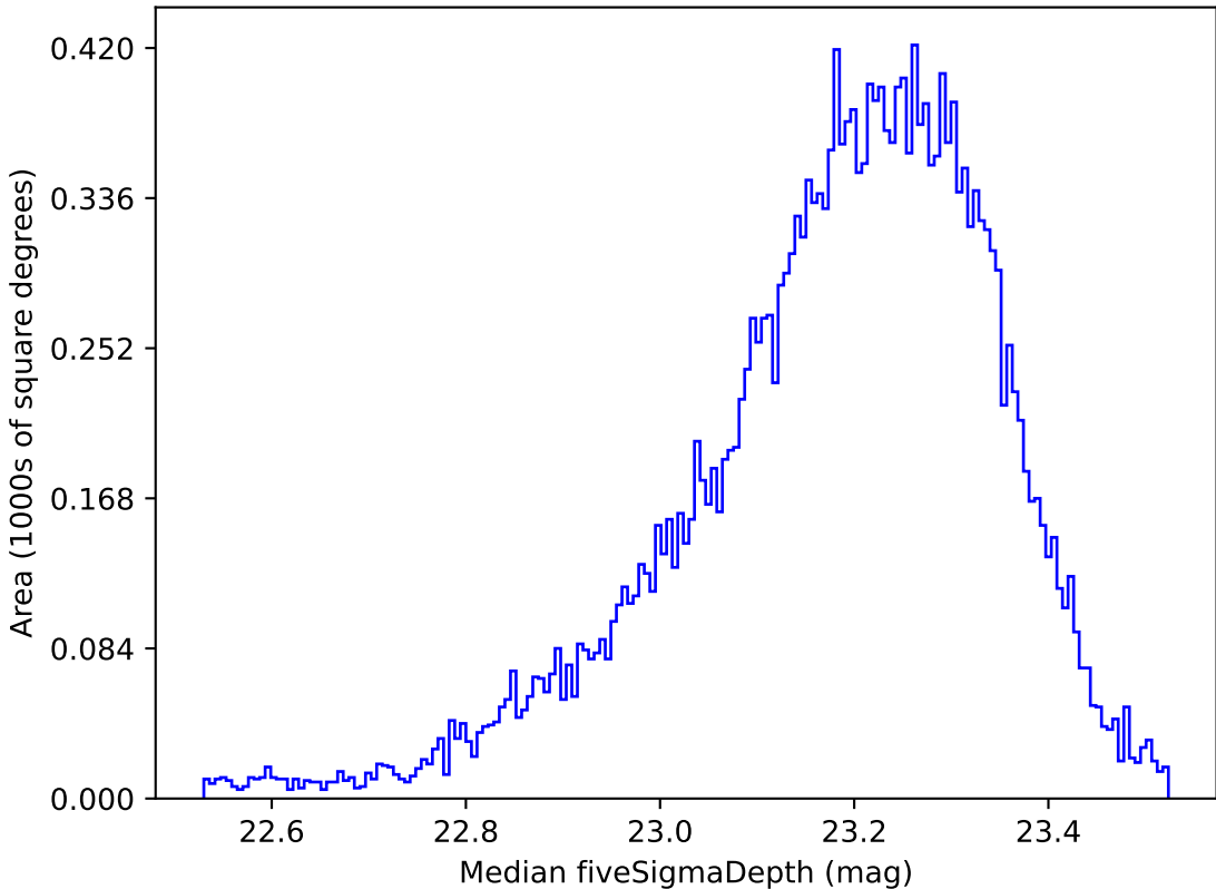
mw_roll_bulge_v3.3_10yrs All sky u band: Median fiveSigmaDepth
