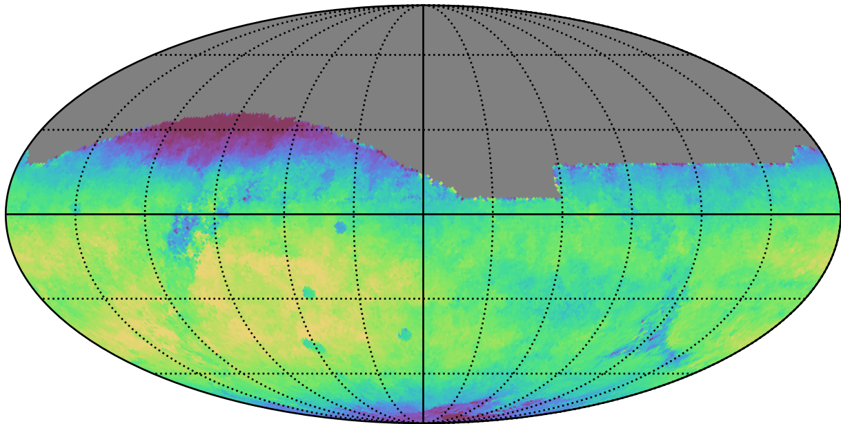
mw_roll_bulge_v3.3_10yrs All sky r band: Median fiveSigmaDepth
