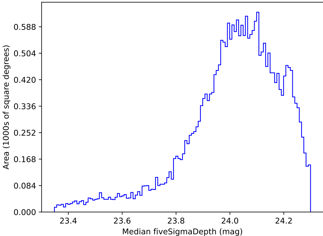
mw_roll_bulge_v3.3_10yrs All sky r band: Median fiveSigmaDepth
