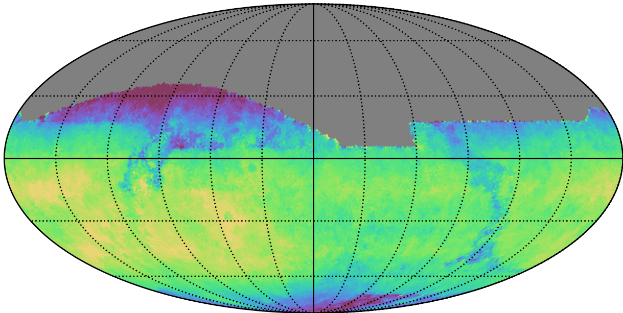
mw_roll_bulge_v3.3_10yrs All sky i band: Median fiveSigmaDepth
