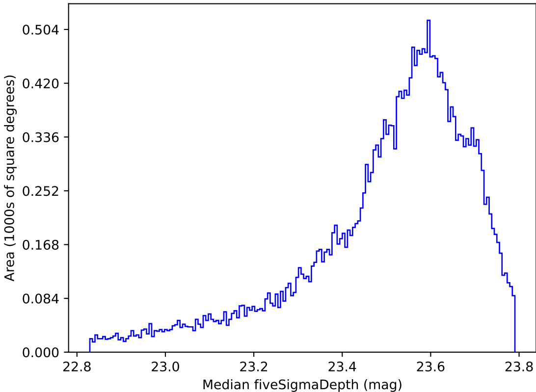
mw_roll_bulge_v3.3_10yrs All sky i band: Median fiveSigmaDepth
