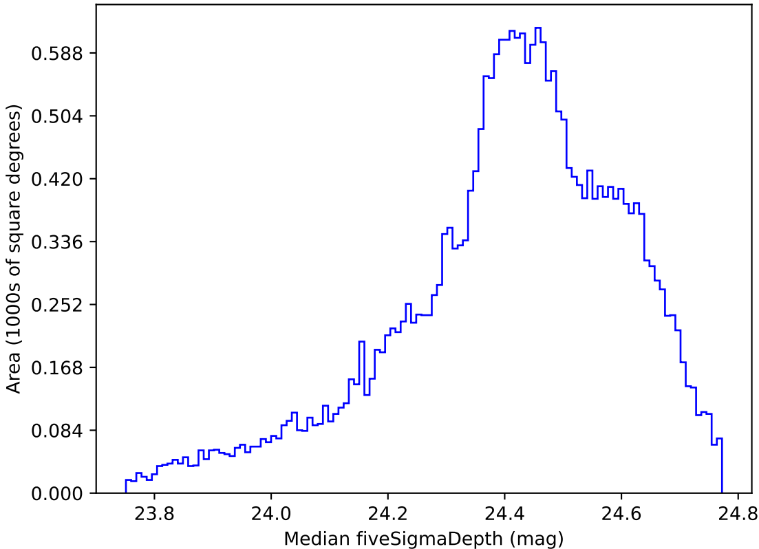
mw_roll_bulge_v3.3_10yrs All sky g band: Median fiveSigmaDepth
