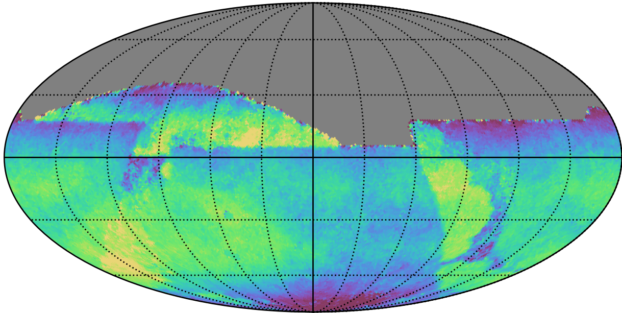
mw_roll_bulge_v3.3_10yrs All sky all bands: Median fiveSigmaDepth
