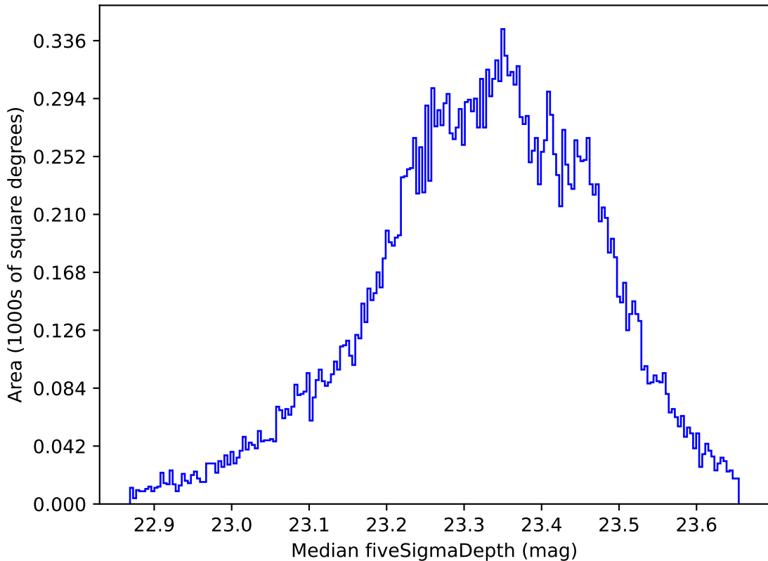
mw_roll_bulge_v3.3_10yrs All sky all bands: Median fiveSigmaDepth
