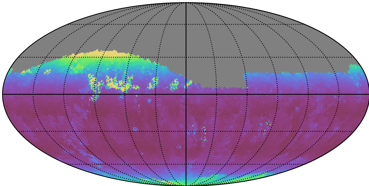
mw_roll_bulge_v3.3_10yrs Yr 1 z band: Median airmass
