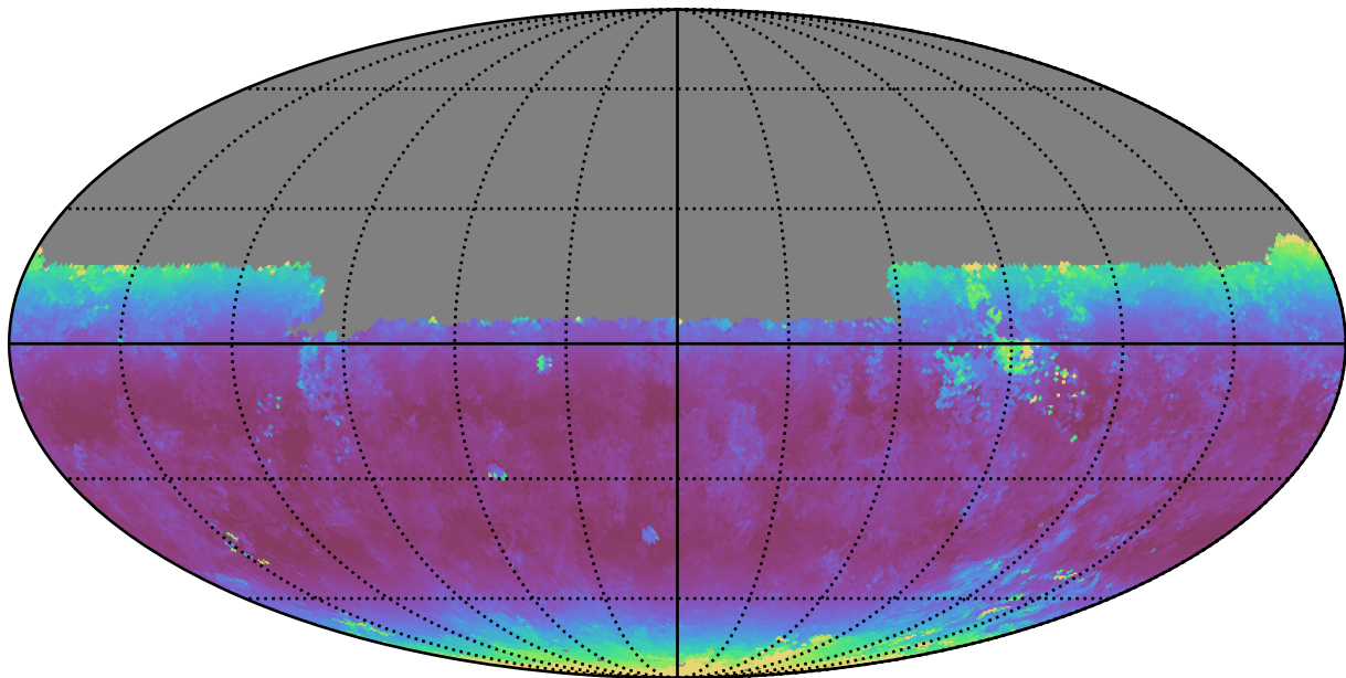
mw_roll_bulge_v3.3_10yrs Yr 1 y band: Median airmass
