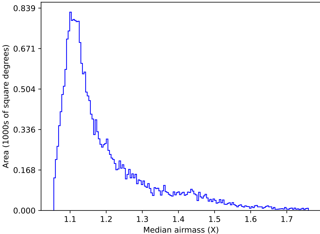
mw_roll_bulge_v3.3_10yrs Yr 1 y band: Median airmass
