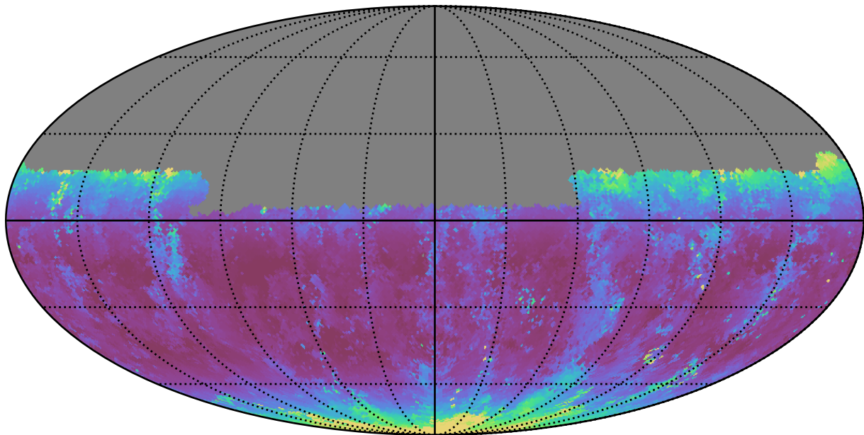
mw_roll_bulge_v3.3_10yrs Yr 1 u band: Median airmass
