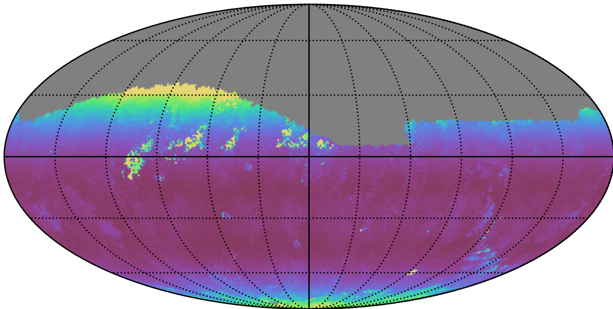
mw_roll_bulge_v3.3_10yrs Yr 1 r band: Median airmass
