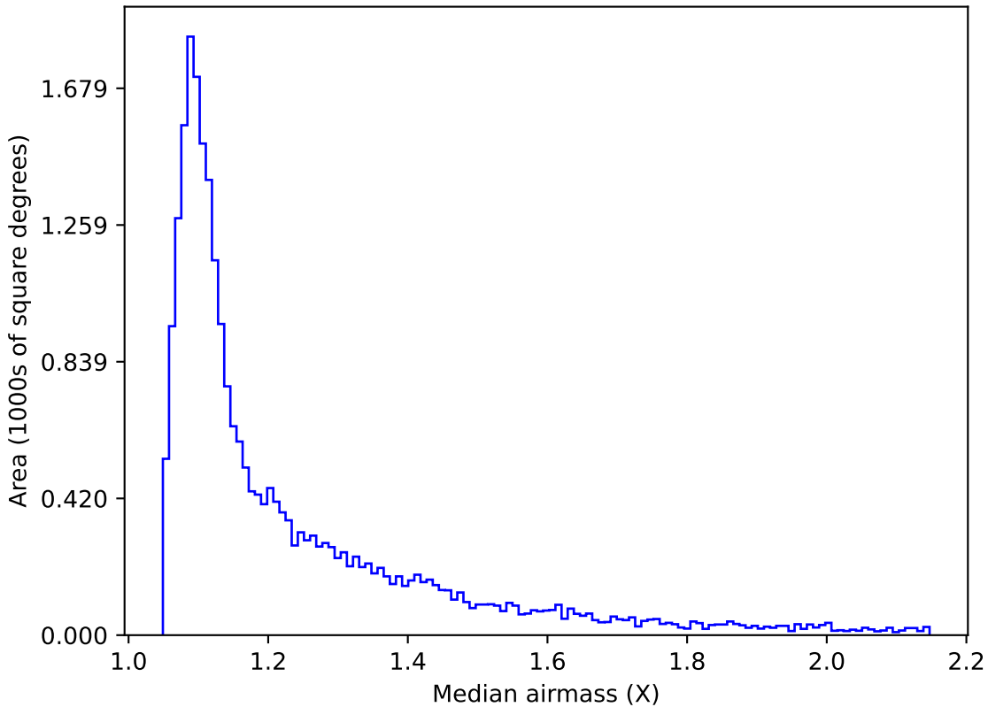
mw_roll_bulge_v3.3_10yrs Yr 1 r band: Median airmass
