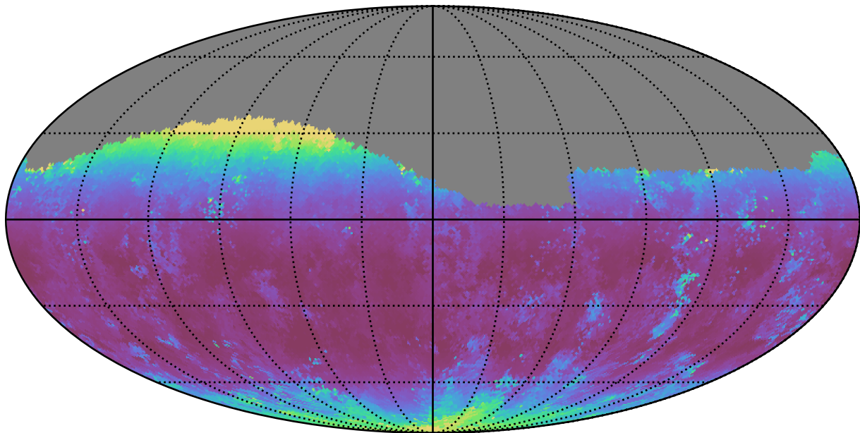
mw_roll_bulge_v3.3_10yrs Yr 1 g band: Median airmass
