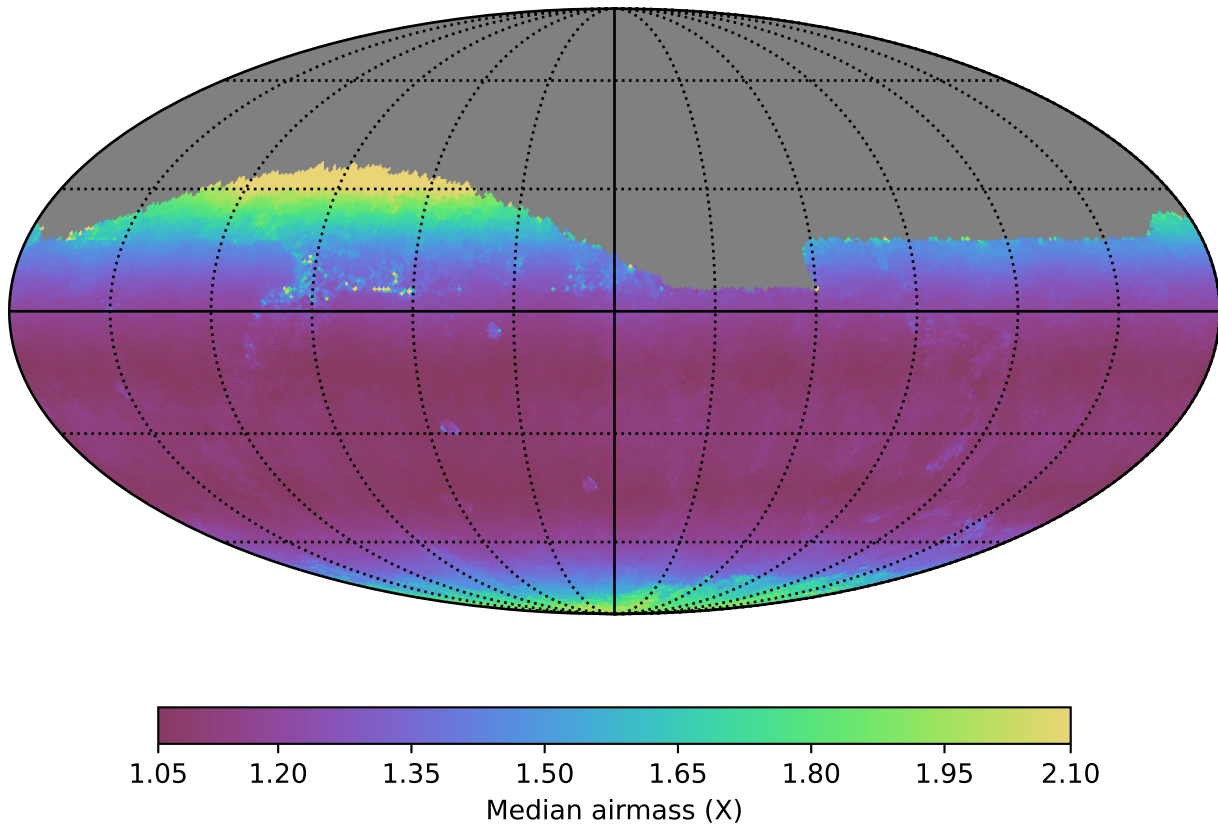
mw_roll_bulge_v3.3_10yrs Yr 1 all bands: Median airmass
